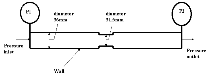
Fig. 3. Geometrical sizes of the experiment facility
