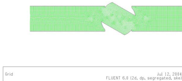
Fig. 4. Typical grid used in CFD analysis
