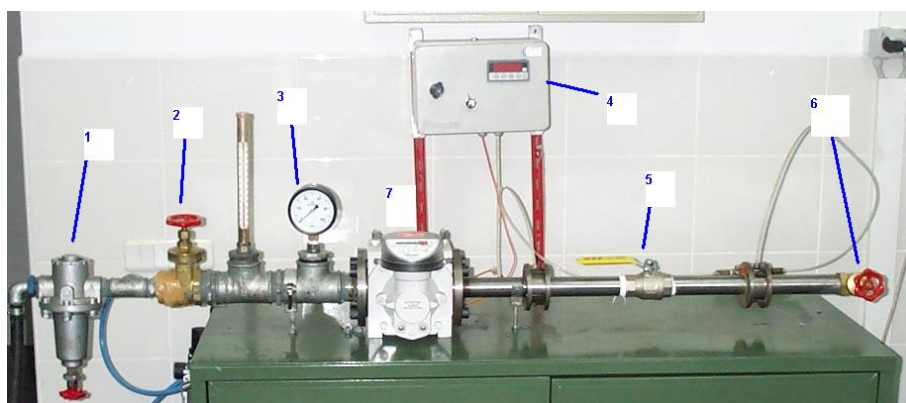
Fig. 2. Experiment facility
