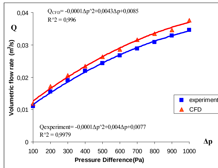
Fig. 12. Relation of pressure drop vs. flow rate
