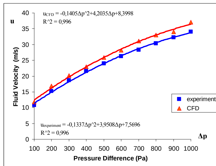
Fig. 13. Relation of pressure drop vs. axial velocity
