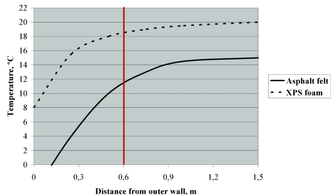
Figure 5 Calculated floor temperature as function of distance from outer wall, using two different seals between sill and concrete slab, (further information in Sandberg and Sikander 2004).
