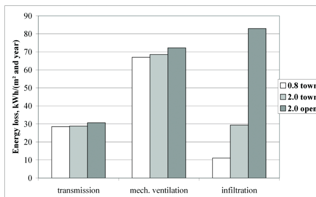
Figure 2 Calculated energy losses for houses with airtightness according to the normal building code (in a town environment) and houses with a below standard airtightness according to the normal building regulations (town environment and open environment).
